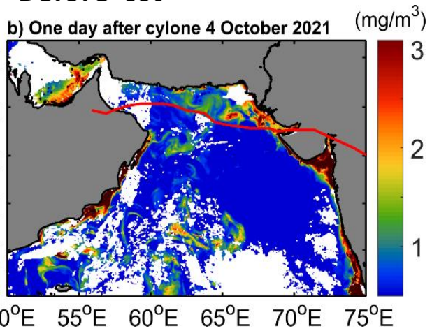
Before chlorophyll-a
