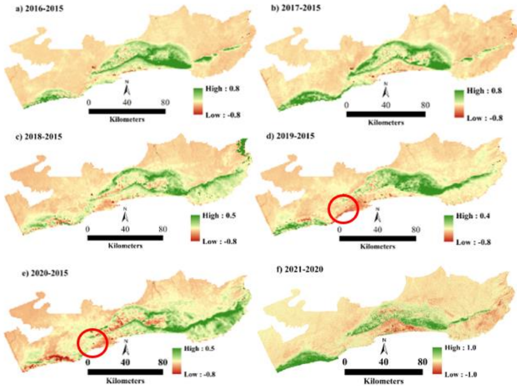
Vegetation index
