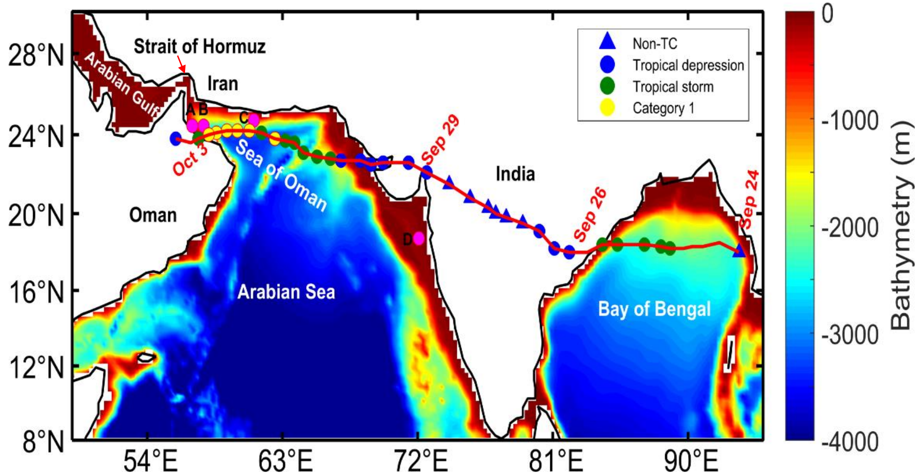
Cyclone track
