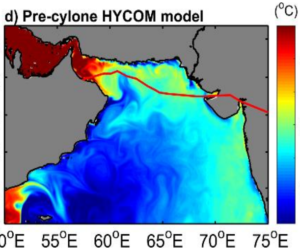
Before sst
