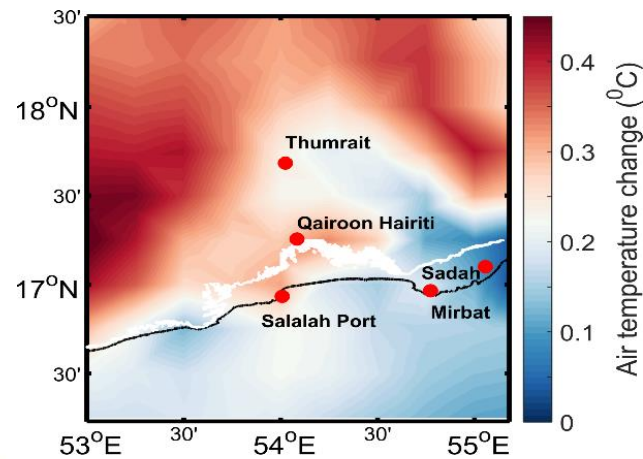
Air temperature
