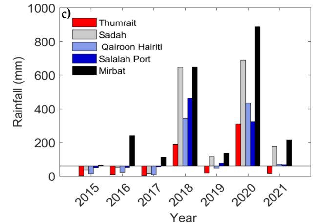
Rainfall
