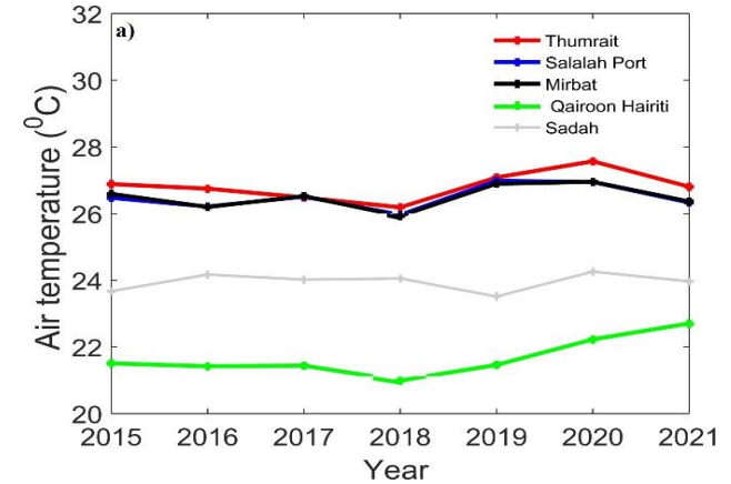
Air temperature
